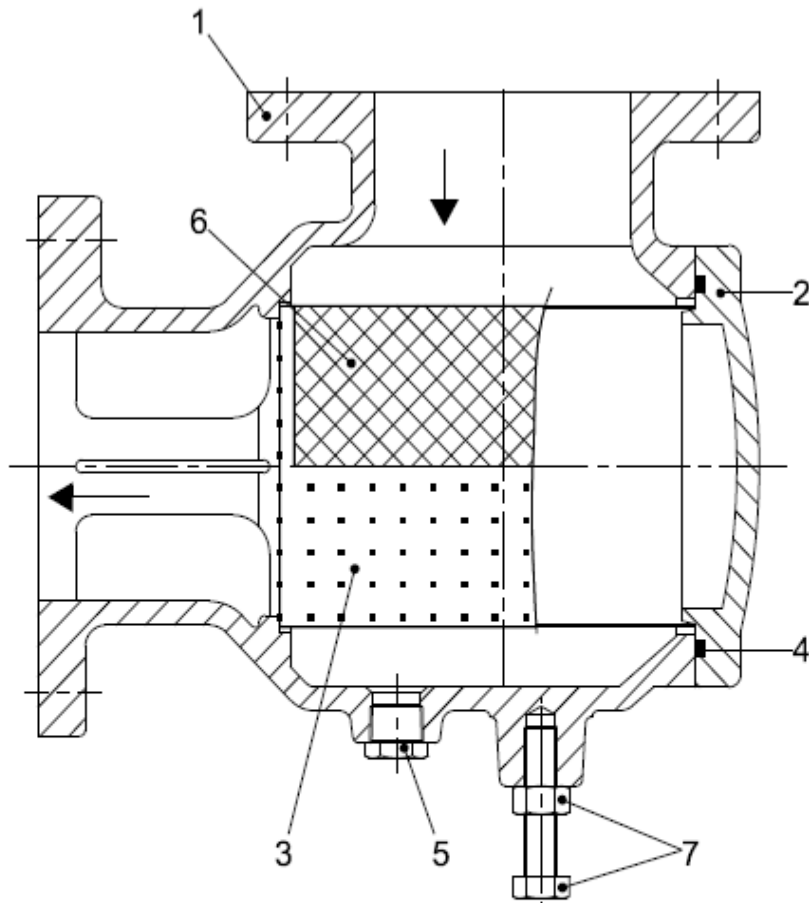
Fig. 3 Sectional drawing of a suction diffuser
